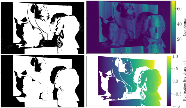
Figure 5: Left: The direct mask only containing pixels with C > 5 (top) and the shadow mask which removes pixels with too little information present (bottom). In both cases, white denotes a retained pixel. Right: The confidence map (top) denotes the ratio between the two highest maxima found in the pixel responses. Based on this information we remove non-reliable pixels from the phase map and only obtain direct pixels (bottom).
