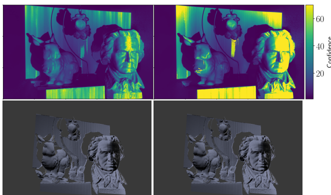
Figure 9: Increasing the number of phases while fixing the number of frequencies results in higher confidence (top) and less artifacts in the reconstructions (bottom). Left: Measurement with 8 equally distributed phase shifts (40 images). Right: Measurement with 16 phaseshifts (80 images).
