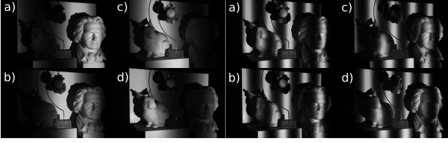
Figure 1: Example images acquired with our illumination procedure. We use sinusoidal illumination patterns with different frequencies ranging from v = 1 (left) to v = 4 (right) and acquire images for four equi-spaced phases in the range [0, 2\pi] (a, b, c, d).
