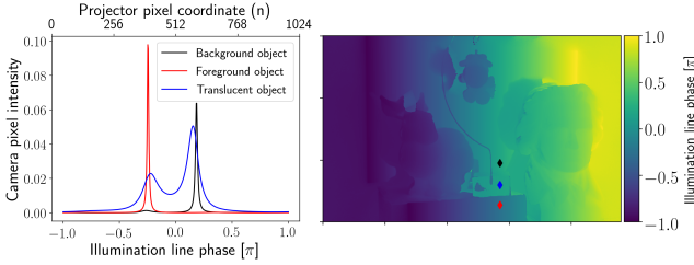
Figure 3: Left: Pixel responses of pixels observing scene points with different objects/materials, corresponding to the color-coded pixels in the right panel. Right: Phase map of the scene depicted in Fig. 1. The estimated phase per pixel corresponds to the global maximum of each camera pixel response.
